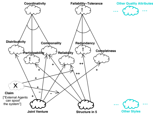
Fig. 8. Partial Evaluation for Organizational Styles
