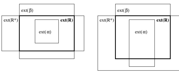
Figure 6: Extensions with and without Hyp 2 .
